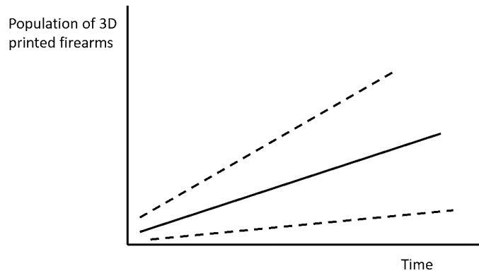
Figure 4. Scenario 3: technological.
