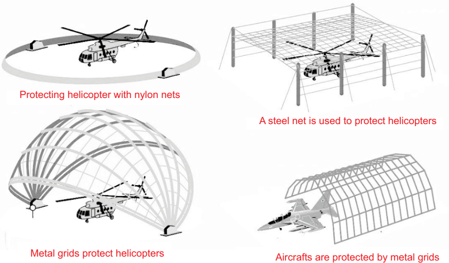
Figure 13. A steel net used to protect military equipment.
